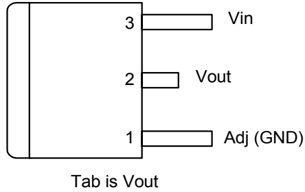
3 PIN TO252
