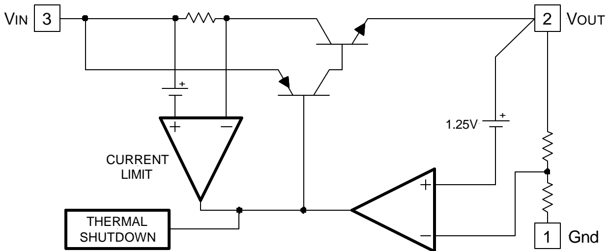
Figure 2 - Simplified block diagram of the APU1030-33.
