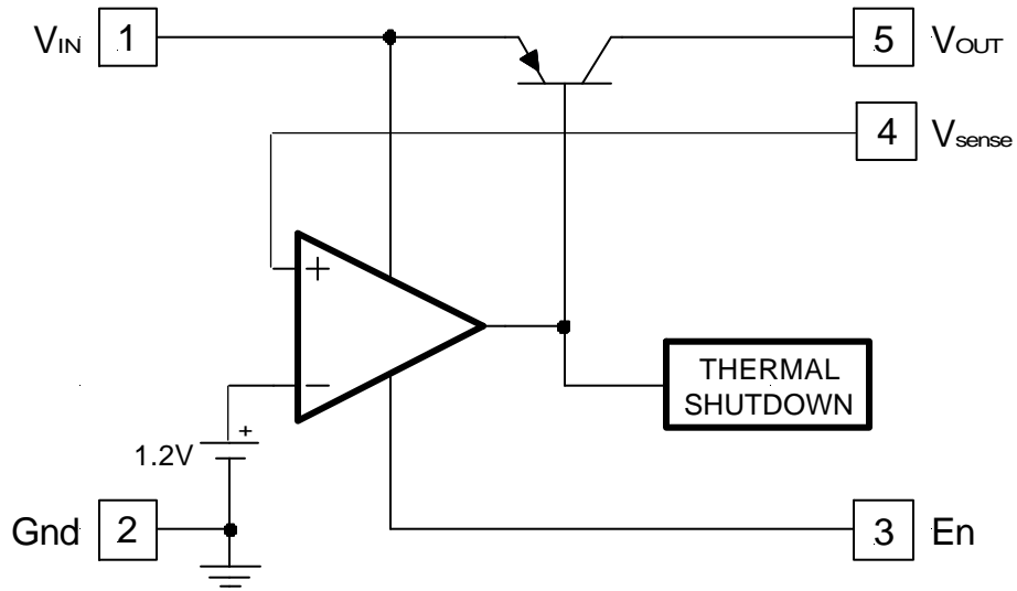
Figure 2 - APU8812 Fixed output 1.2V block diagram.
