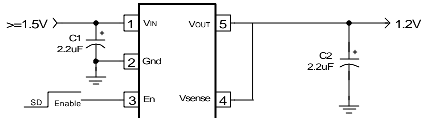
Figure 1 - Typical application of the APU8812 fixed voltage regulator.
