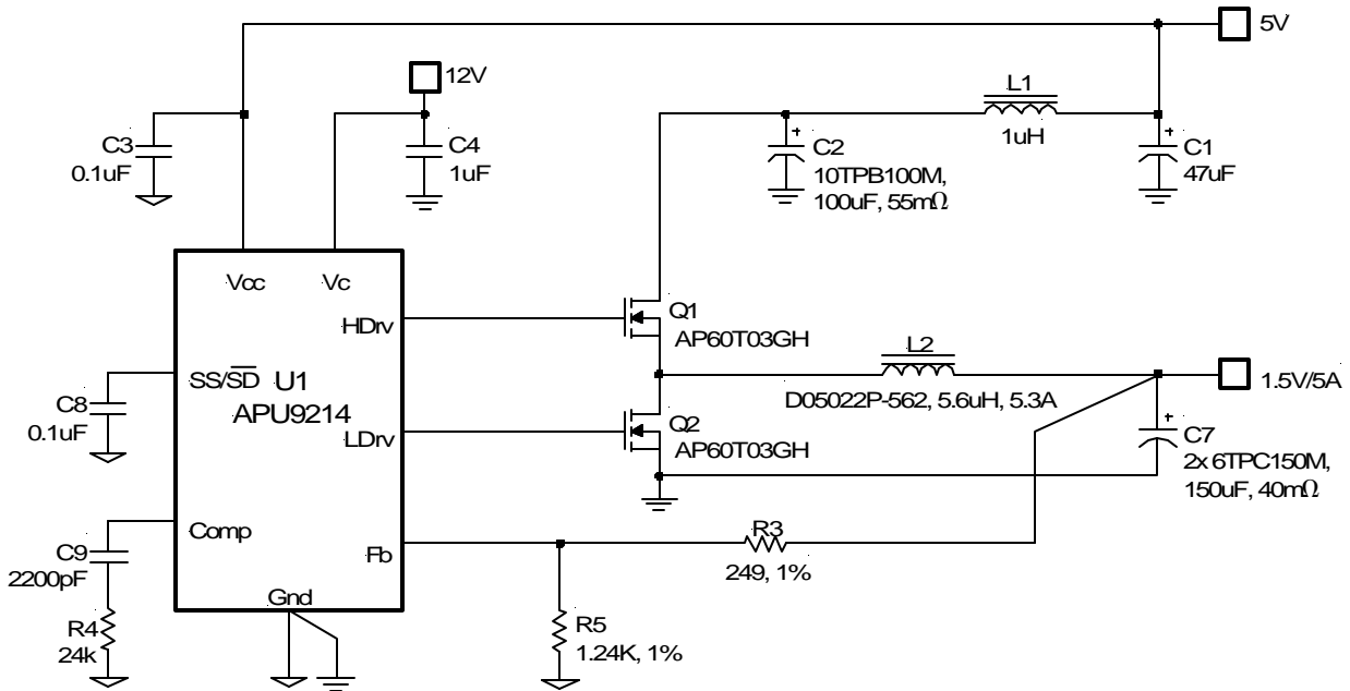
Figure 1 - Typical application of APU9214 or APU9214A.
