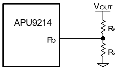
Figure 3 - Typical application of the APU9214 for programming the output voltage.
