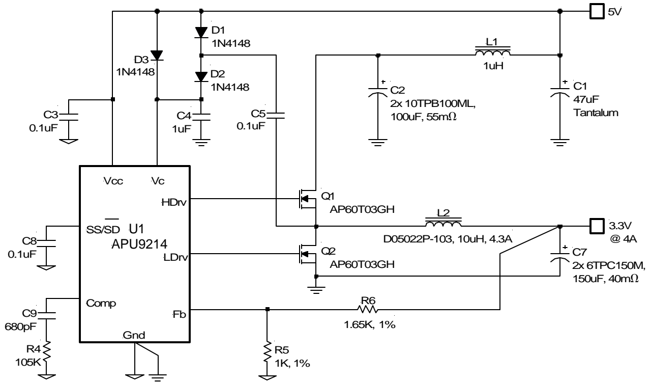
Figure 18 - Typical application of APU9214 in an on-board DC-DC converter using a single 5V supply.
