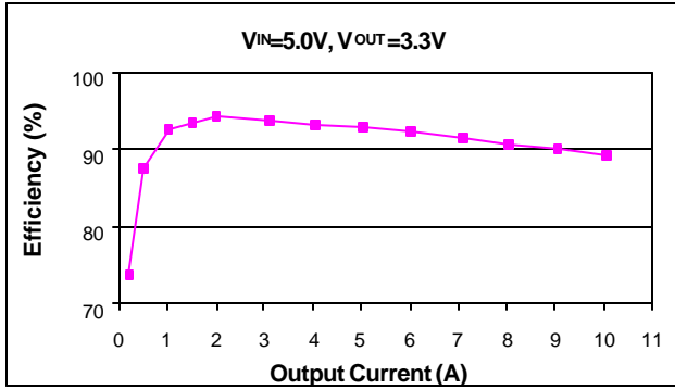
Figure 22 - Efficiency for APU9214 Evaluation Board.
