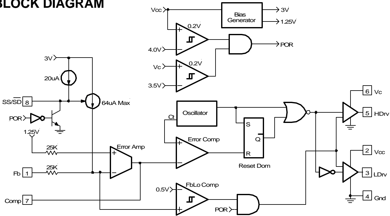
Figure 2 - Simplified block diagram of the APU9214.
