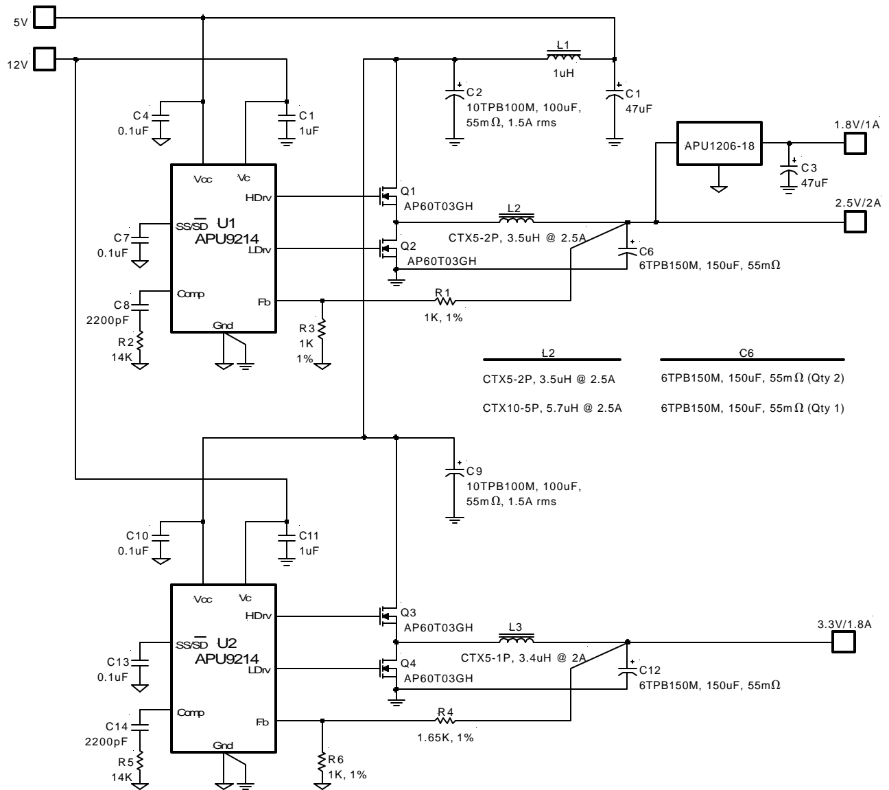
Figure 19 - Typical application of APU9214 or APU9214A in an on-board DC-DC converter providing the Core, GTL+, and Clock supplies for the Pentium II microprocessor.
