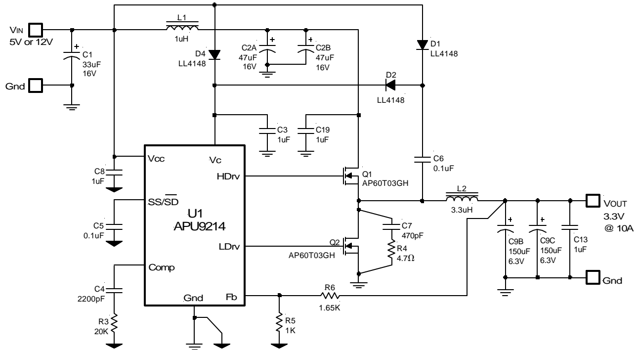
Figure 21 - Demo-board application of APU9214.
