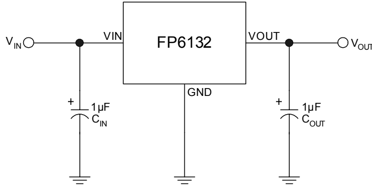
Figure 2. Typical Application Circuit of FP6132
