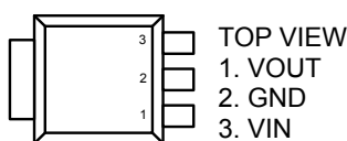
Figure 1. Pin Assignment of FP6132
