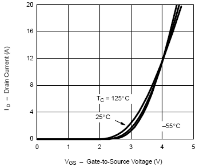
Transfer Characteristics
